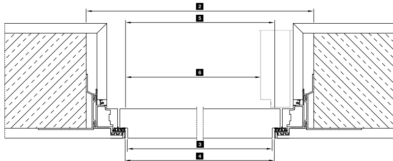
Horizontal view with reverse-opening door leaf
