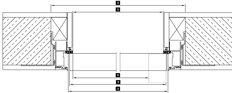
Horizontal view with flush door leaf
