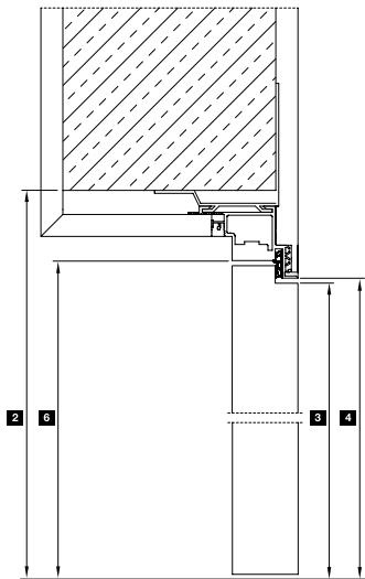
Vertical view with reverse-opening door leaf
