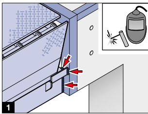
Rear view pit model P with angle profile, delivery including lifting equipment
