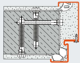
Fitting with grouting lugs
