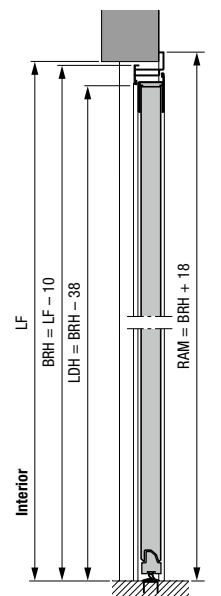
Side door with aluminium corner frame, profile type 2 External fitting
